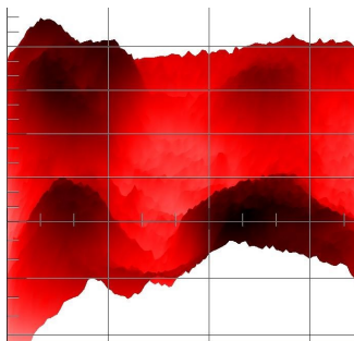
Detection of four delaminations in a fresco
