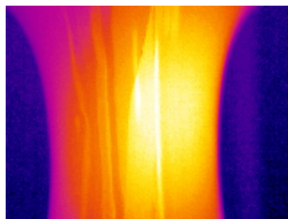
Detection of a crack in an ovoid ceramics vase
