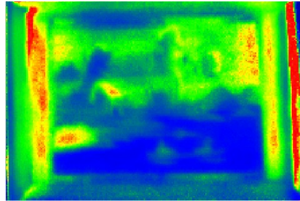
Detection of delaminations in a marquetry
